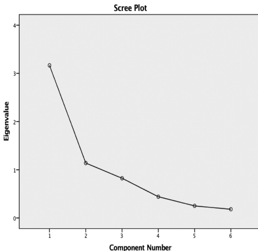
Figure 2 Scree plot. inspection of the scree plot indicated that the inflection point occurred after the second component, or NBP, was extracted using a direct oblimin rotation.
